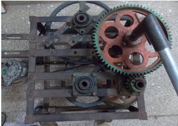
Fig. 1: Human powered mechanical device.
